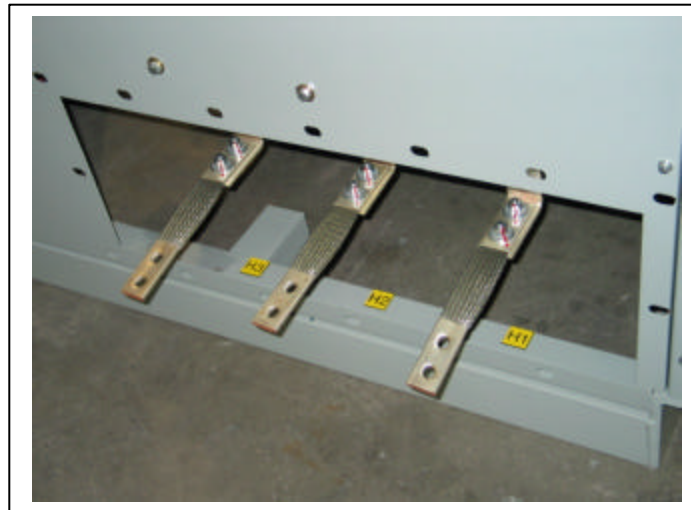
Typical 15kV class transformer - switchgear connection
